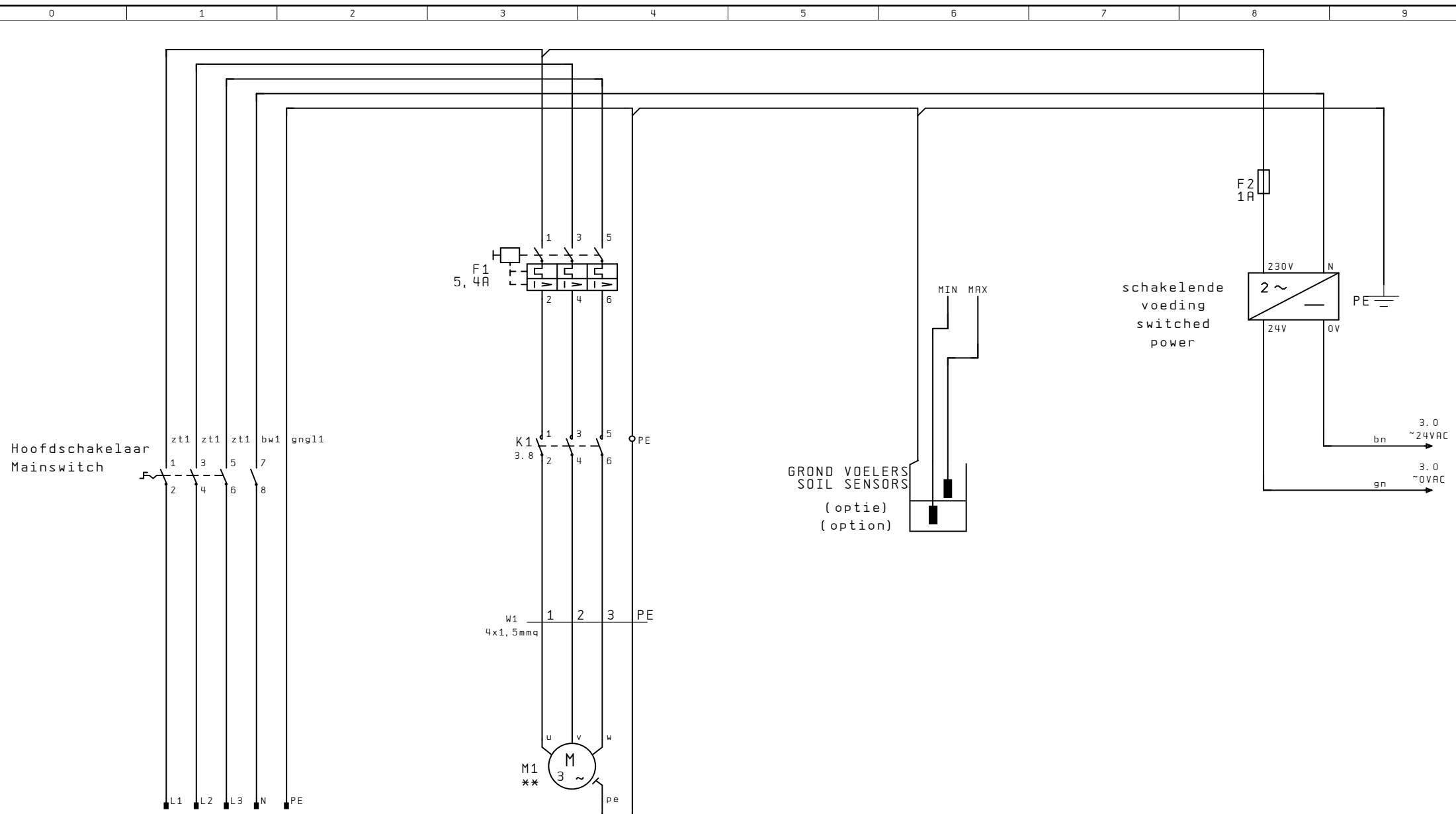
Voeding Power 3~400V+PE-50/60Hz
